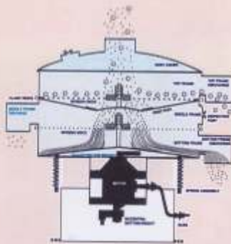
Schematic of Typical Two - 1 DECK Vibroscreen Circular Separator
